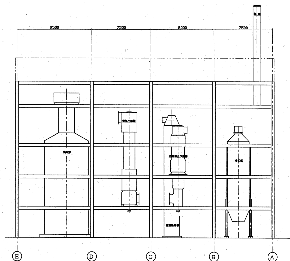
SECTION B-B
