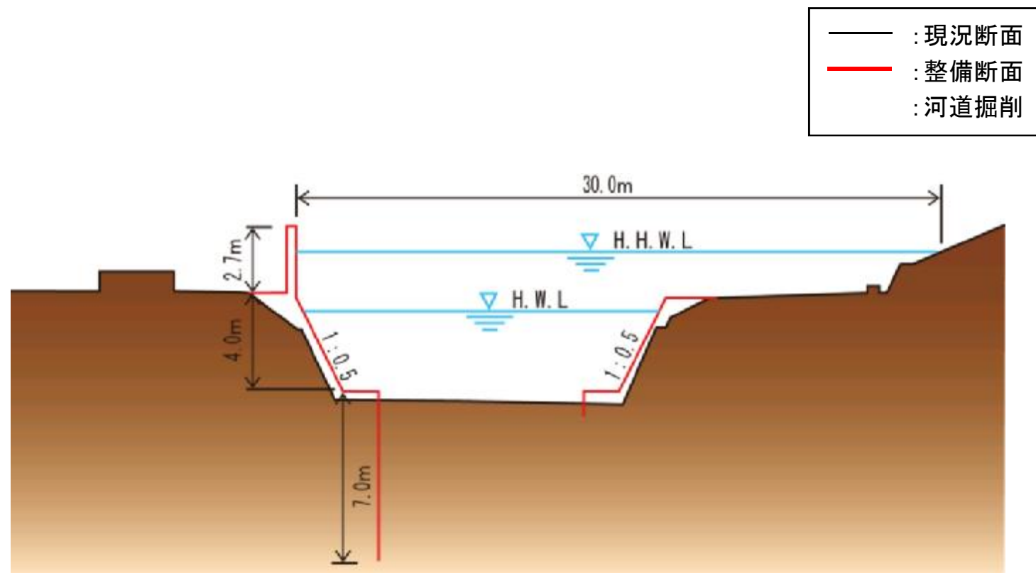
整備断面例 (0.5km地点)
